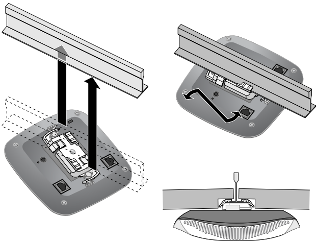
Figure 8 Mounting the AP
