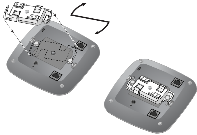
Figure 7 Attaching the Ceiling Rail Adapter
