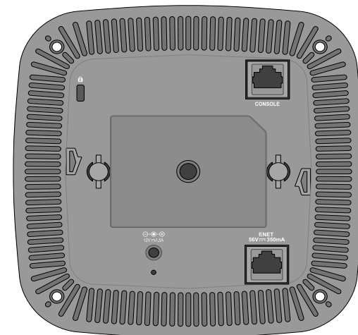
Figure 3 W-AP200 Series Bottom View
